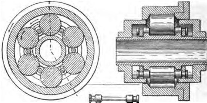
FIG. 463. —Sectional Diagrams of the "American" Roller Bearing. These bearings are beveled at the ends, as indicated, the bevels taking up the end thrusts, and are separated by smaller rollers, one of which is shown below the larger figures. These separating rollers do not come into contact with the rotating axle.
